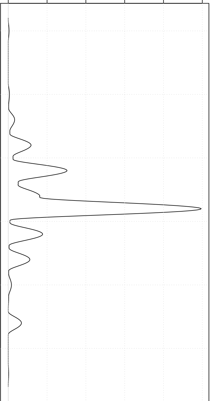
Biweight Kernel
