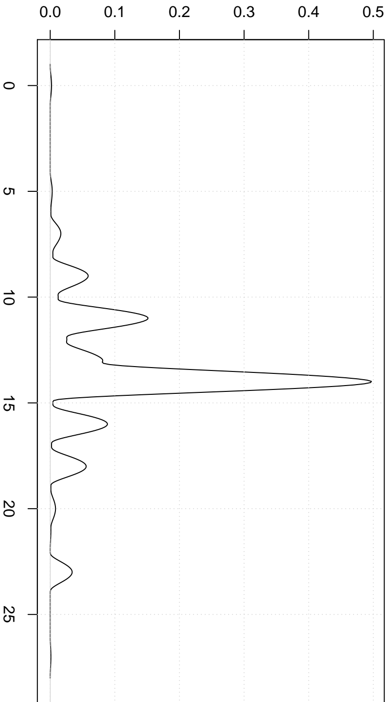
Biweight Kernel
