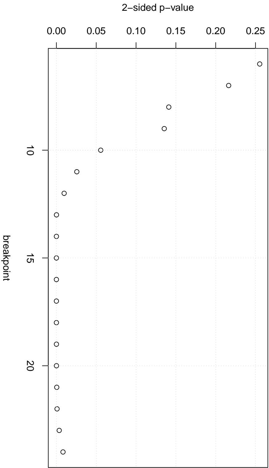
Goldfeld-Quandt test
