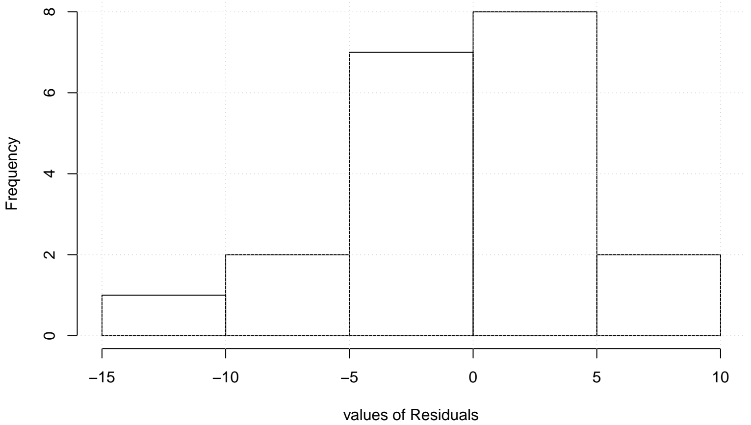
Residual Histogram
