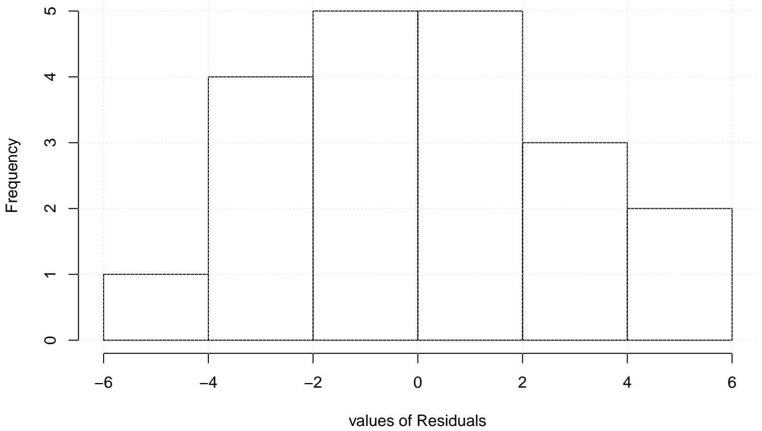
Residual Histogram
