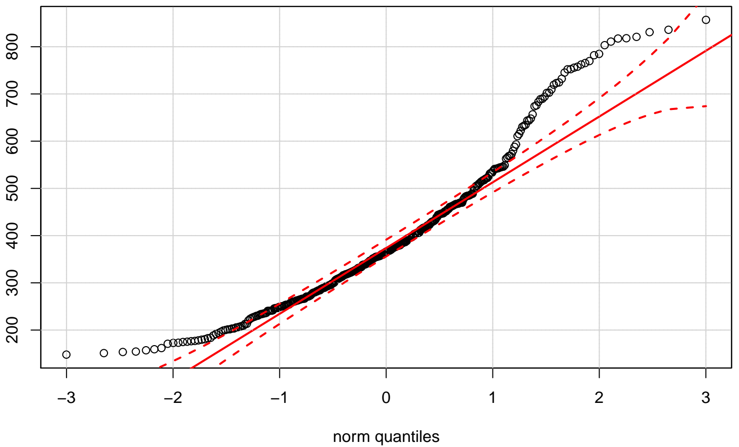
QQ plot (Normal) with confidence intervals
