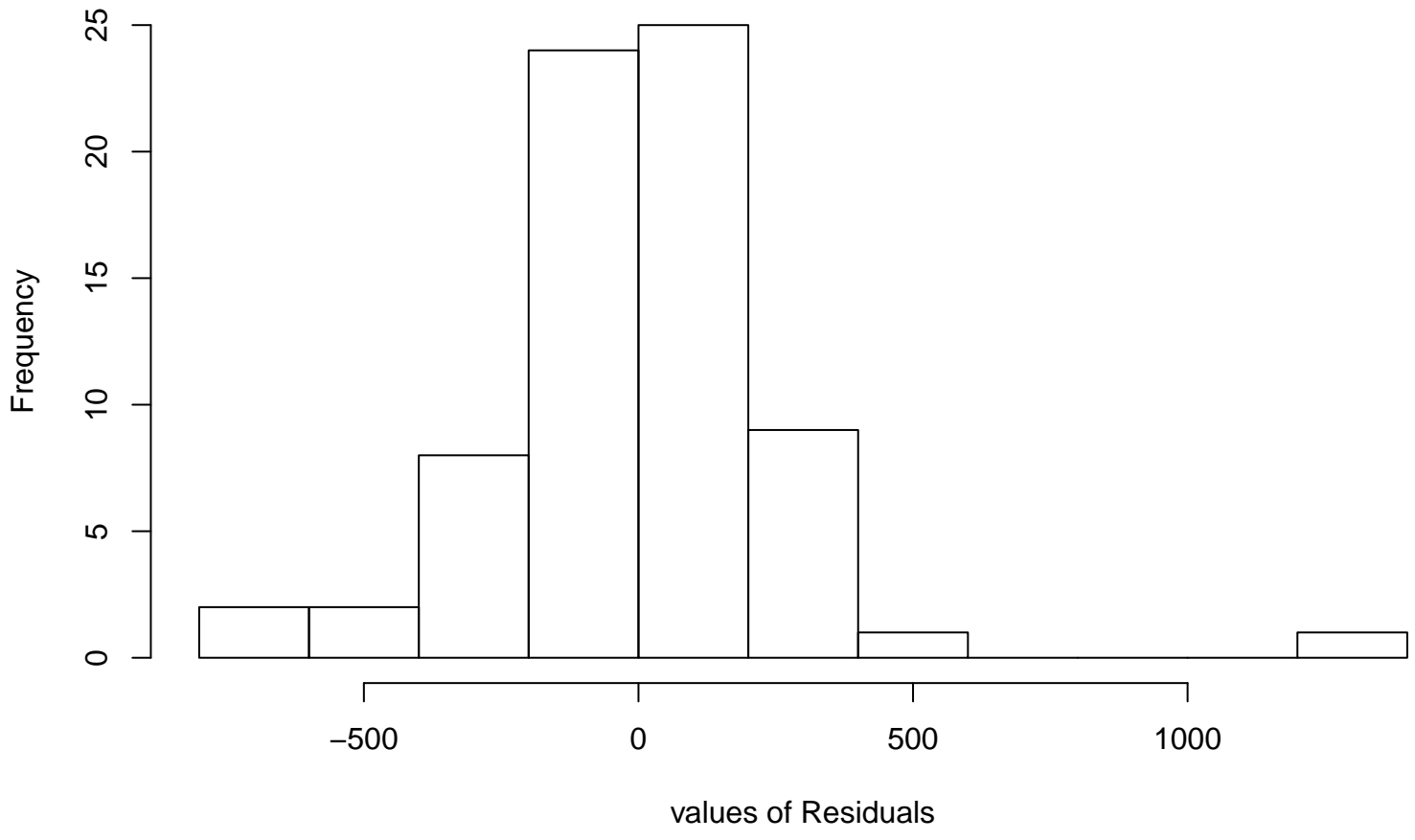
Residual Histogram
