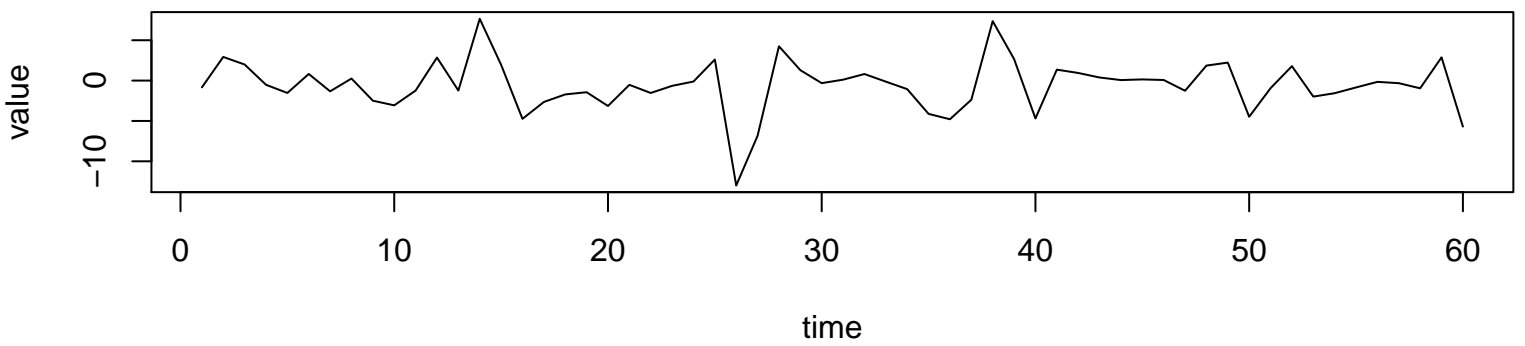
Working Time Series (lambda=0.4, d=0, D=1)
