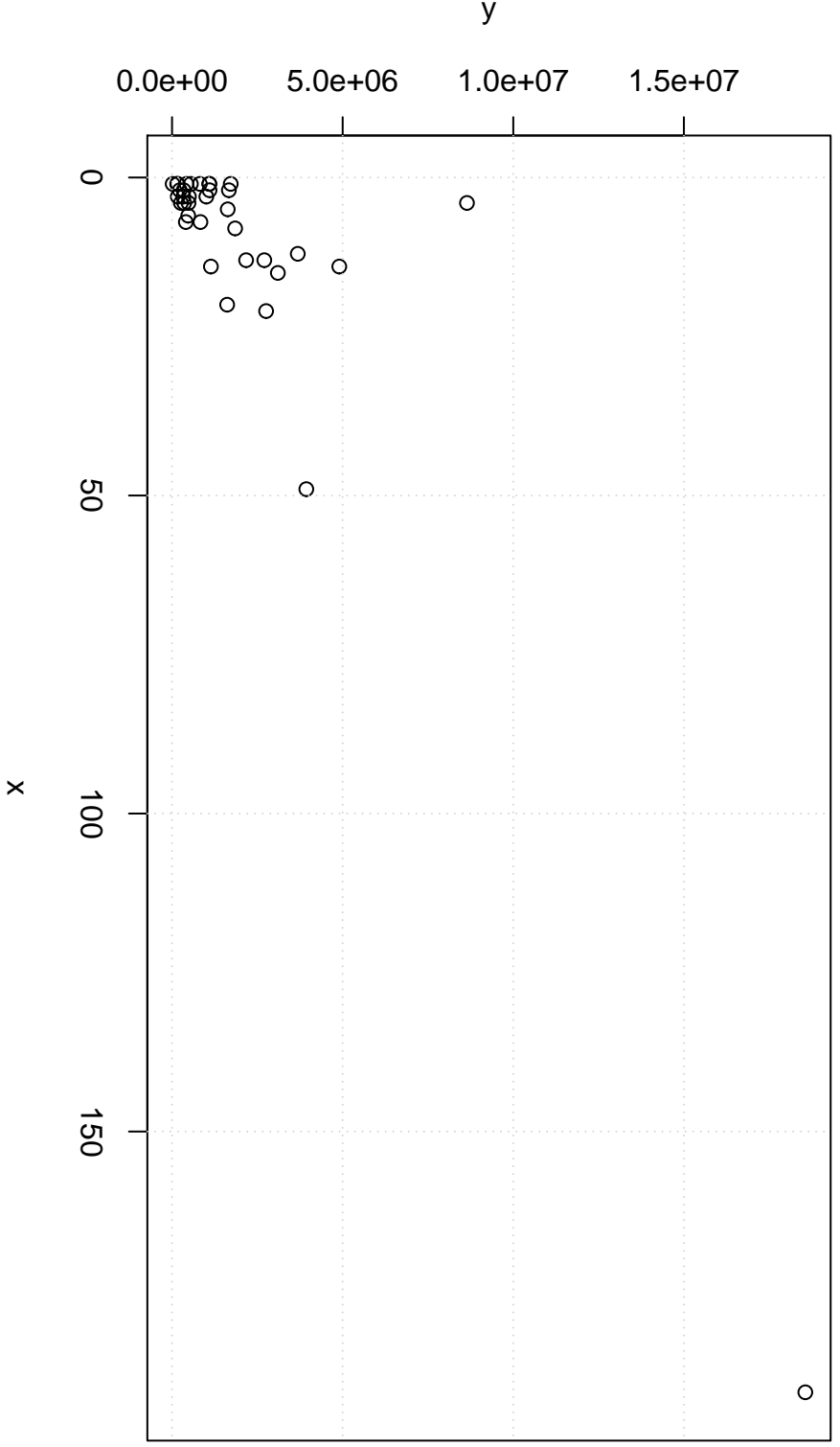
Scatterplot
