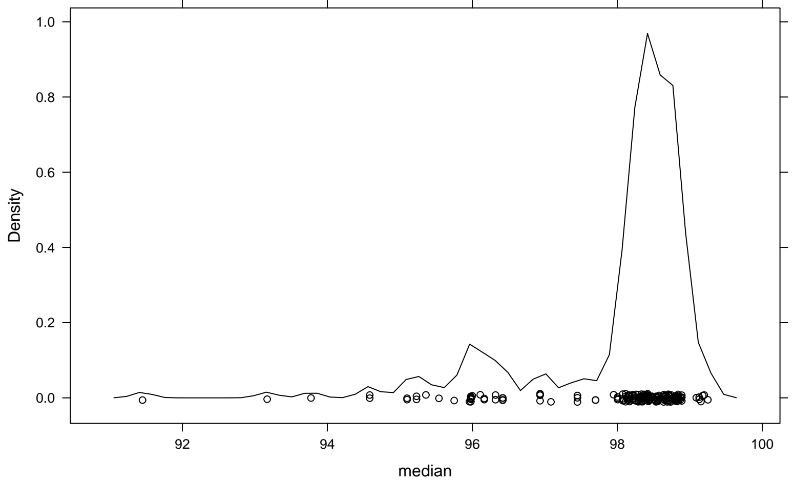
Density Plot
