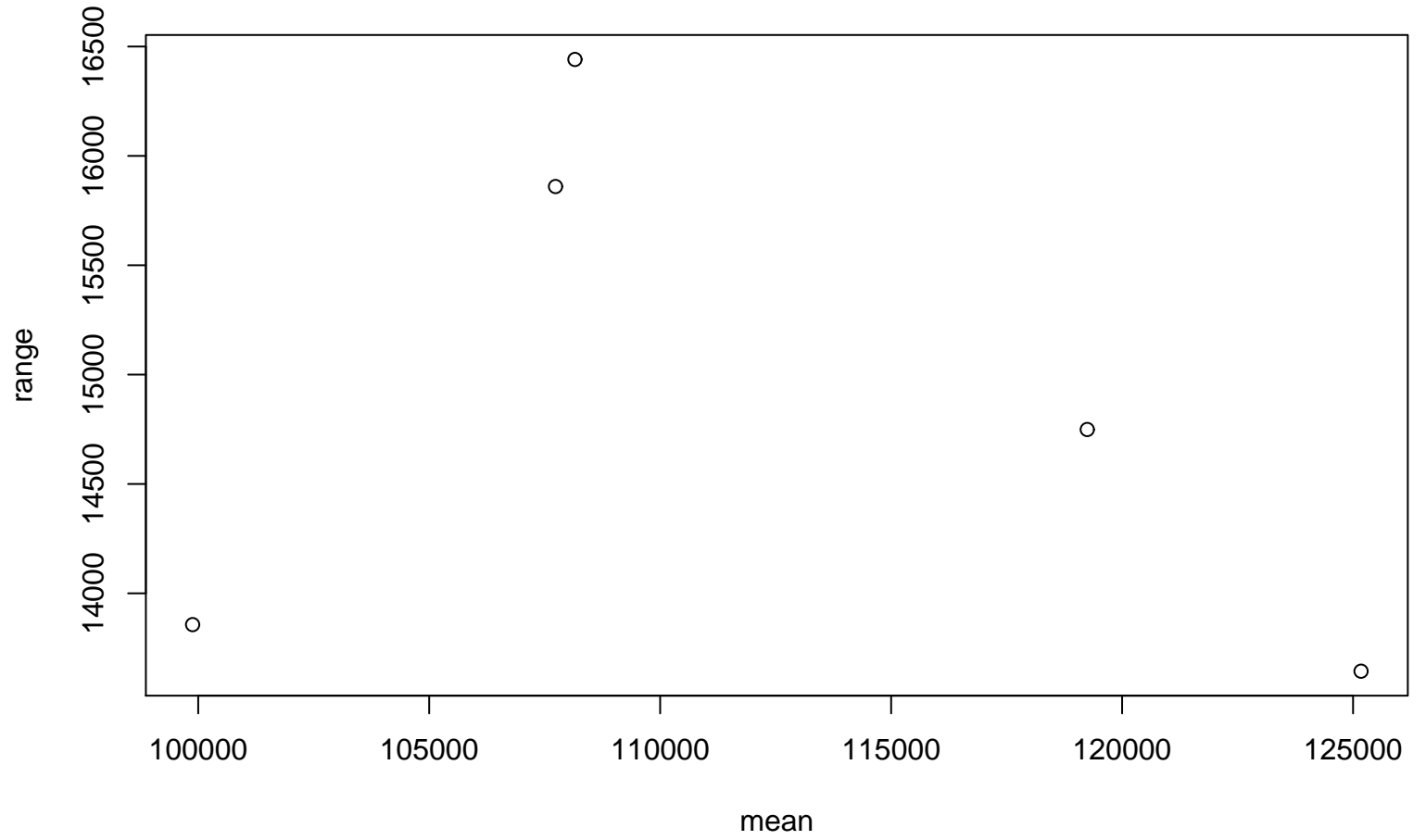
Range-Mean Plot
