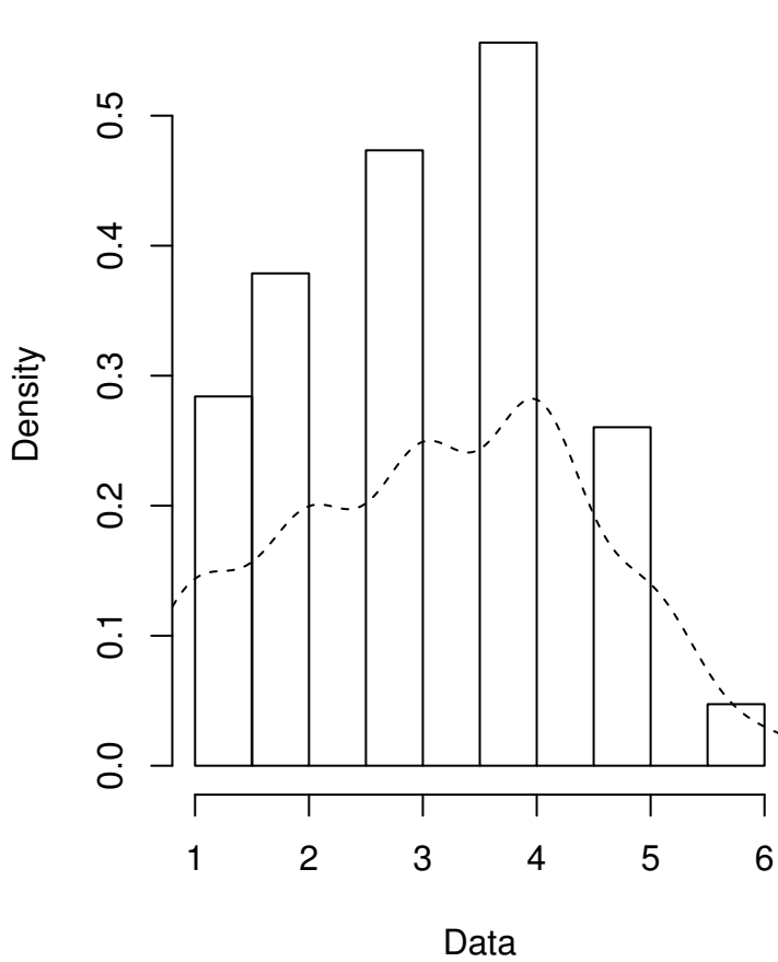
Empirical density
