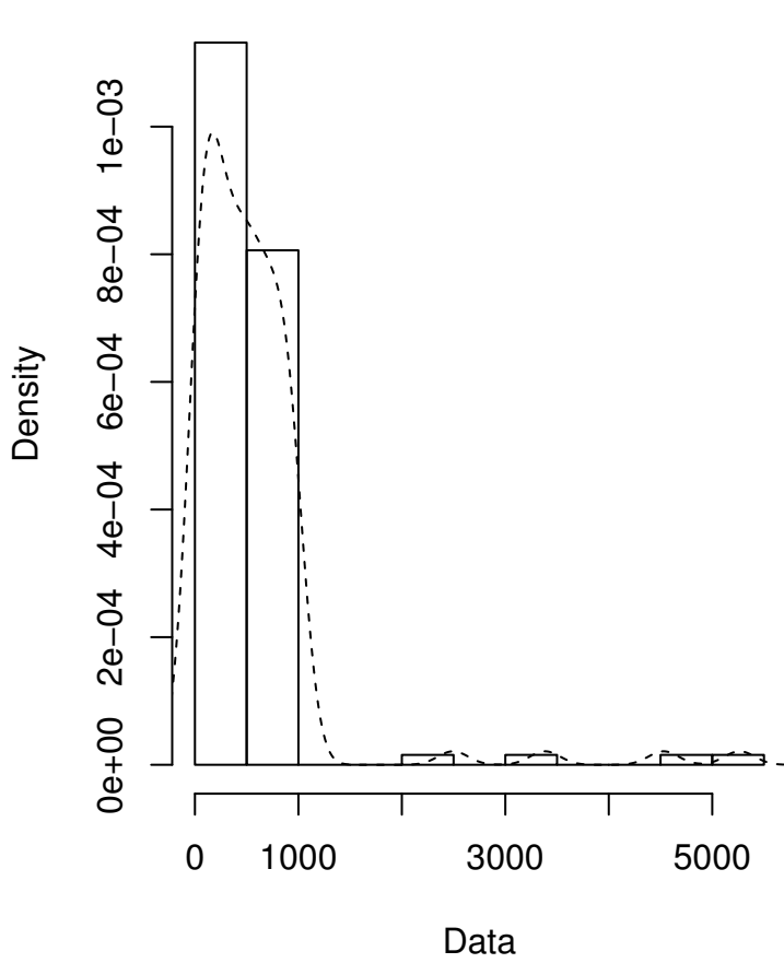
Empirical density
