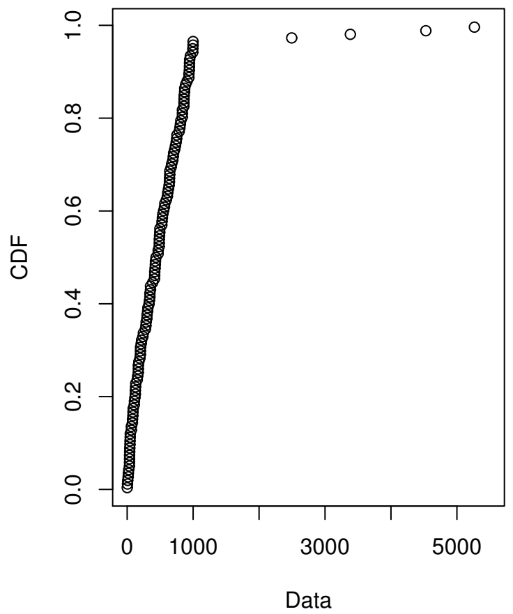
Cumulative distribution
