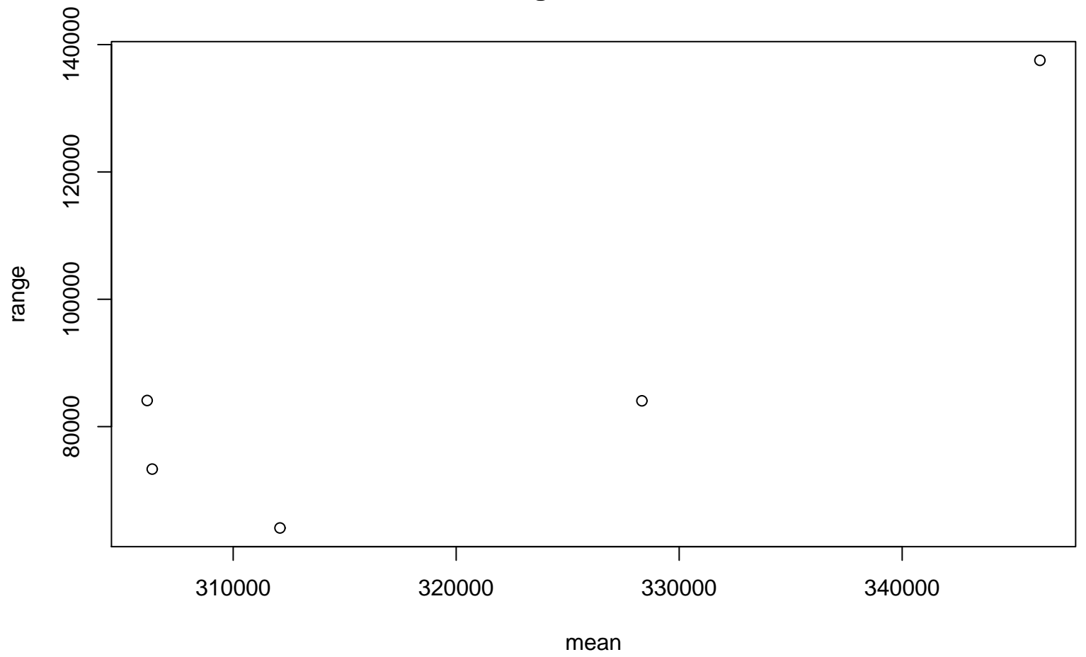
Range-Mean Plot
