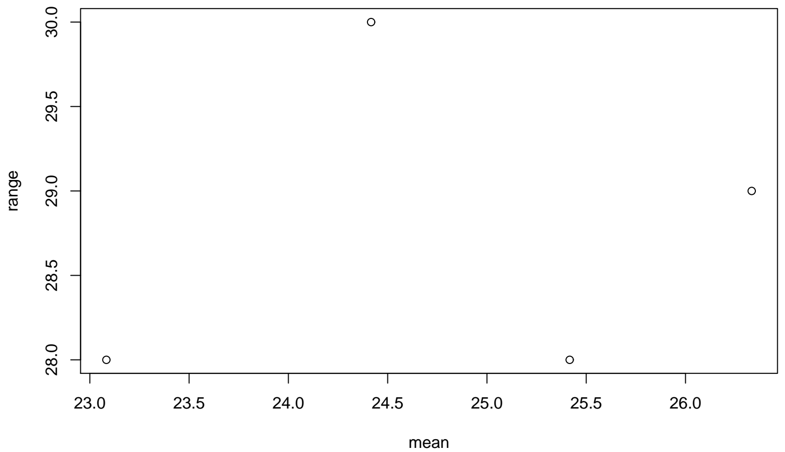
Range-Mean Plot
