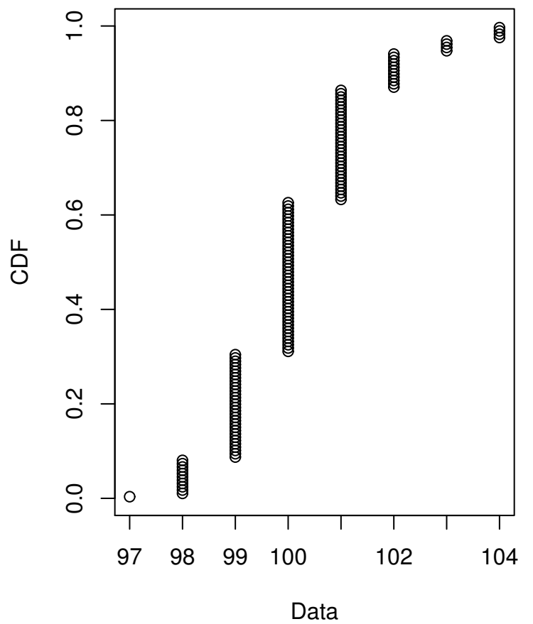
Cumulative distribution
