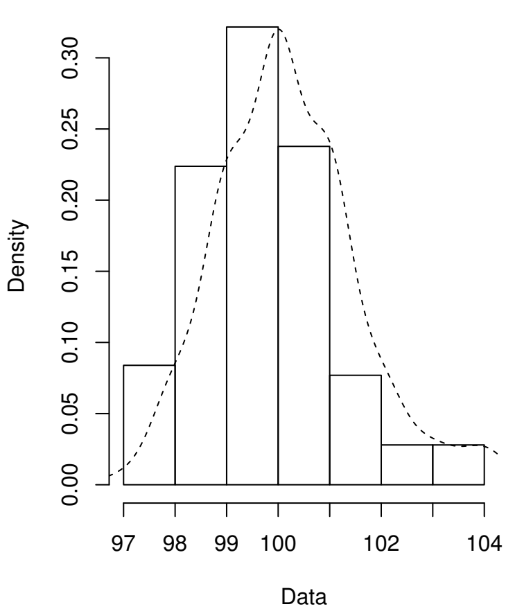
Empirical density
