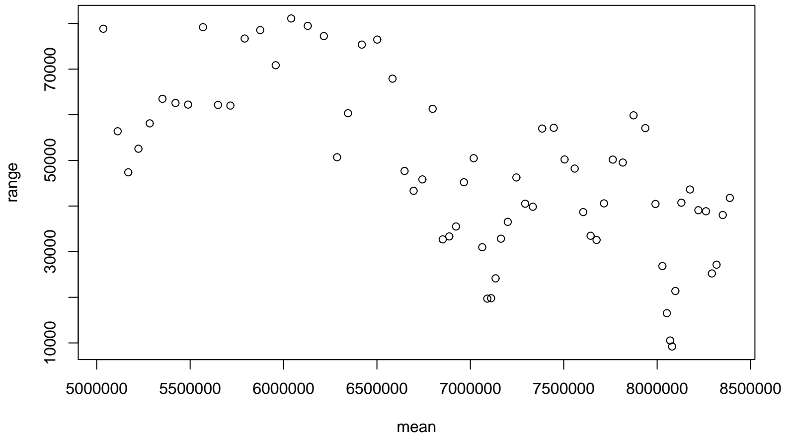
Range-Mean Plot
