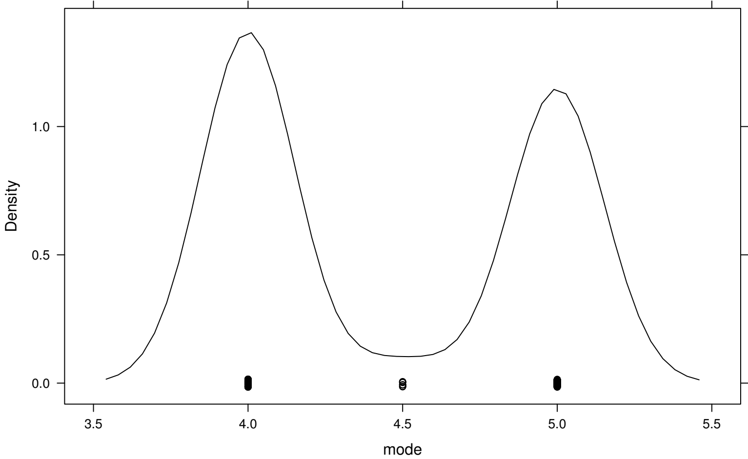
Density Plot
