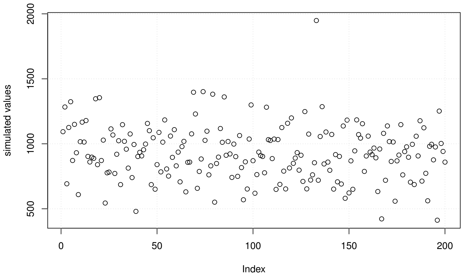
Simulation of Mode of Kernel Density
