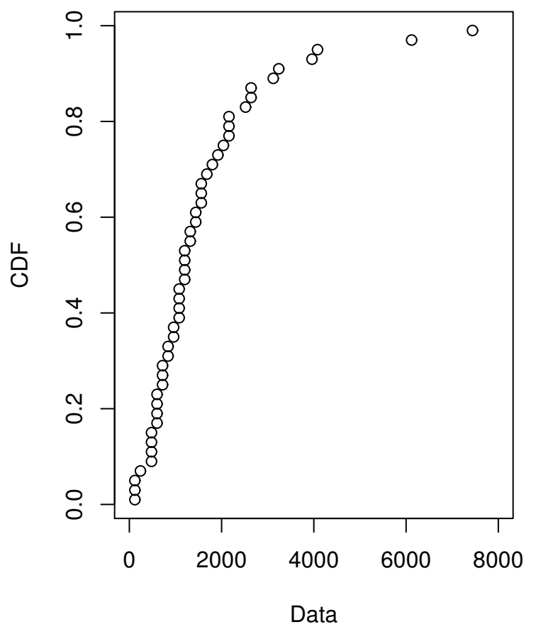
Cumulative distribution
