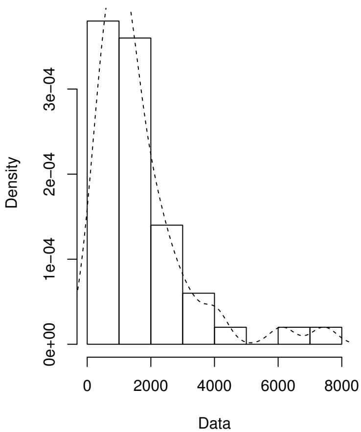
Empirical density
