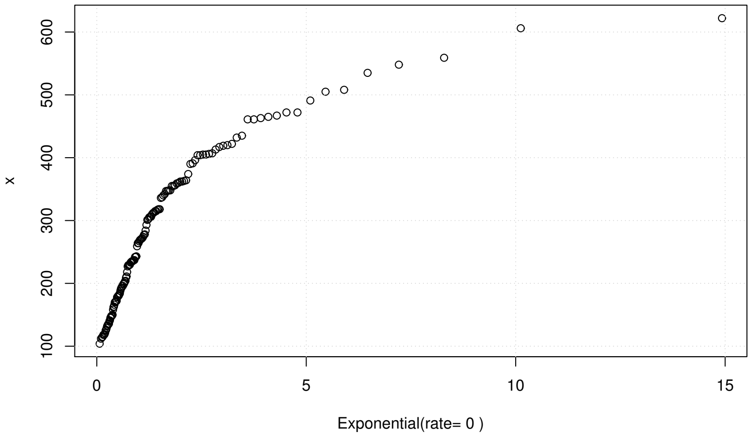
QQ plot (Exponential)
