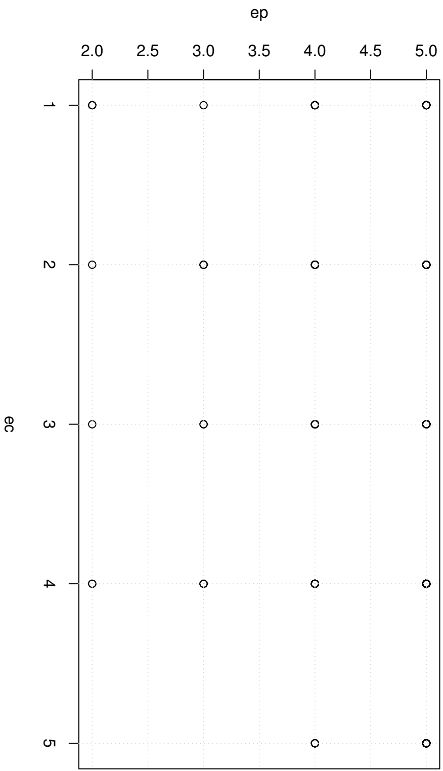
Scatterplot
