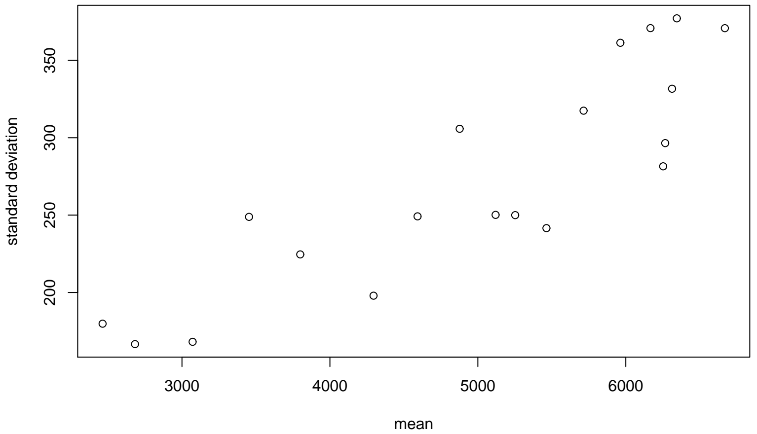
Standard Deviation–Mean Plot
