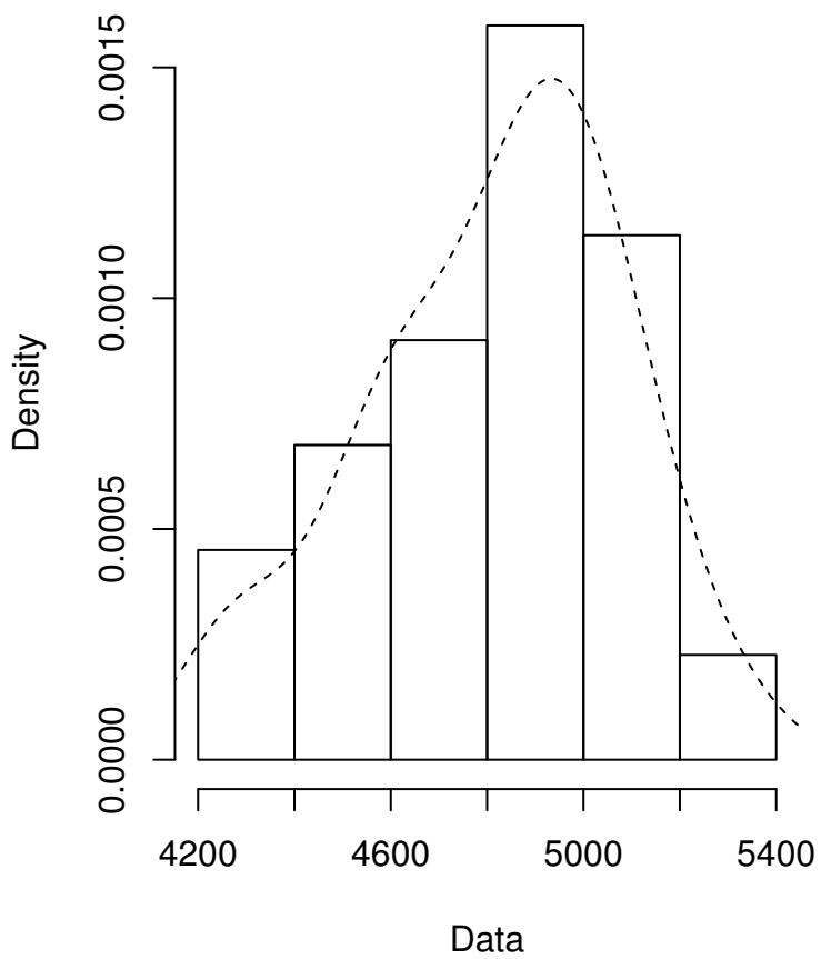
Empirical density
