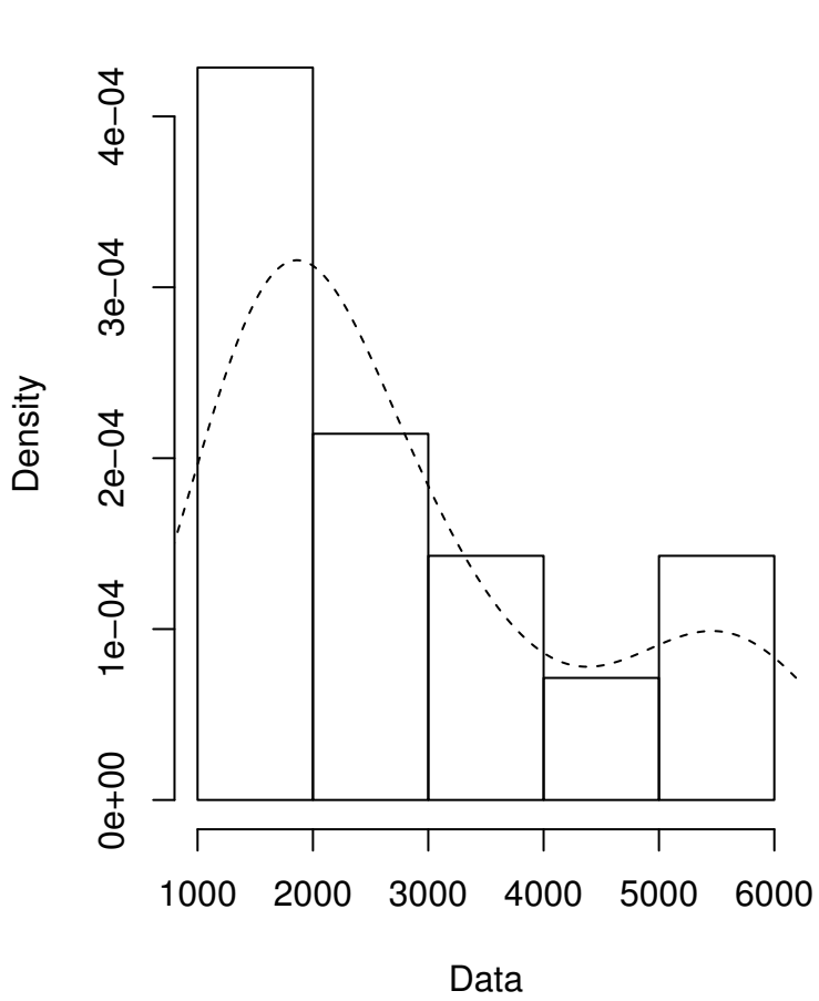
Empirical density
