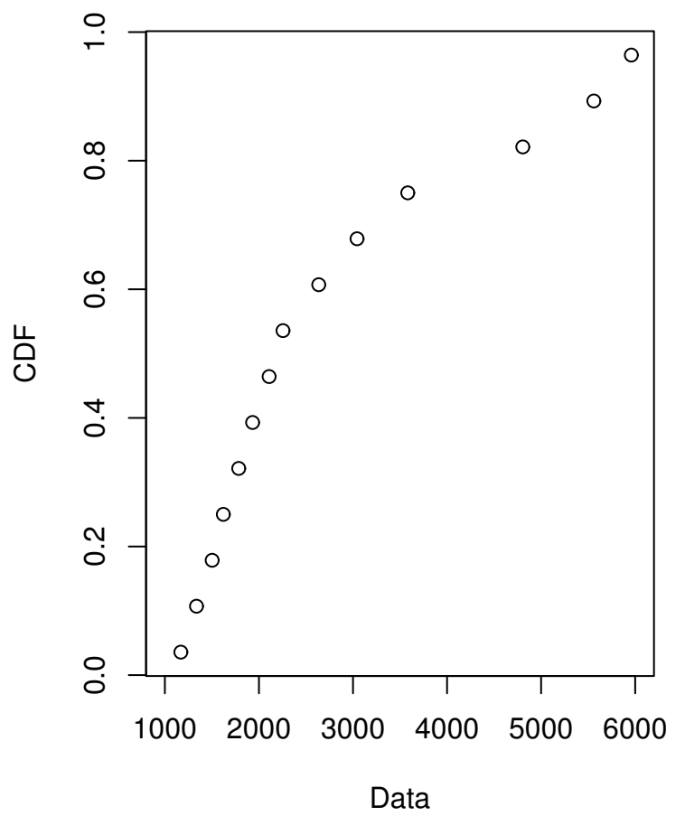
Cumulative distribution
