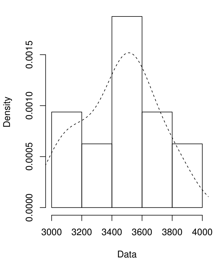
Empirical density
