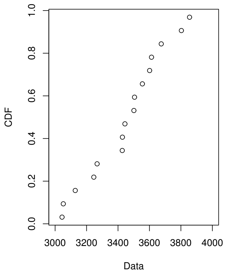
Cumulative distribution
