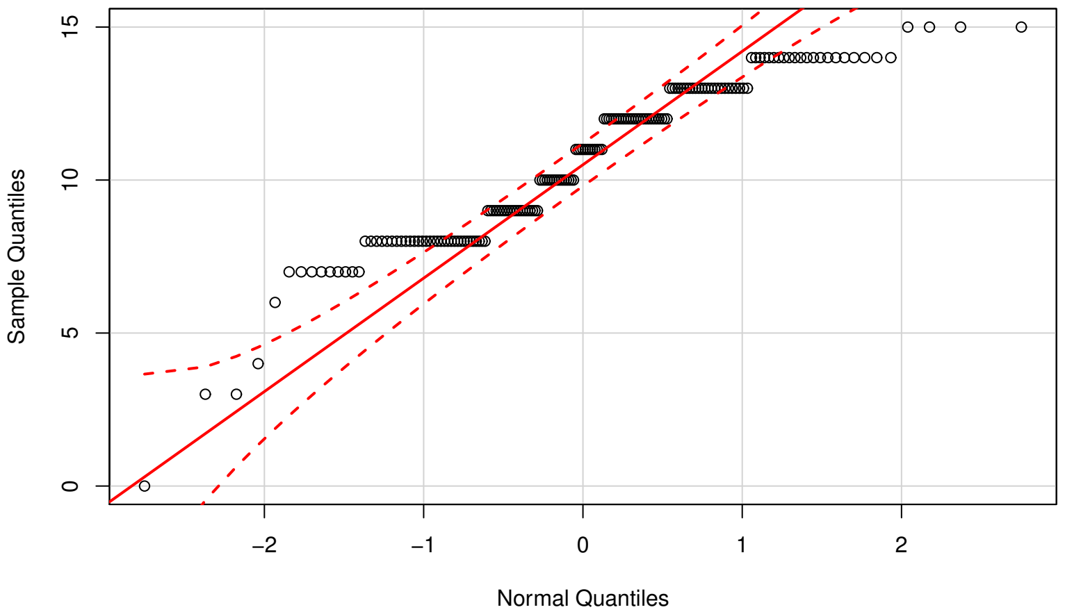
Normal Q-Q Plot (series Y)
