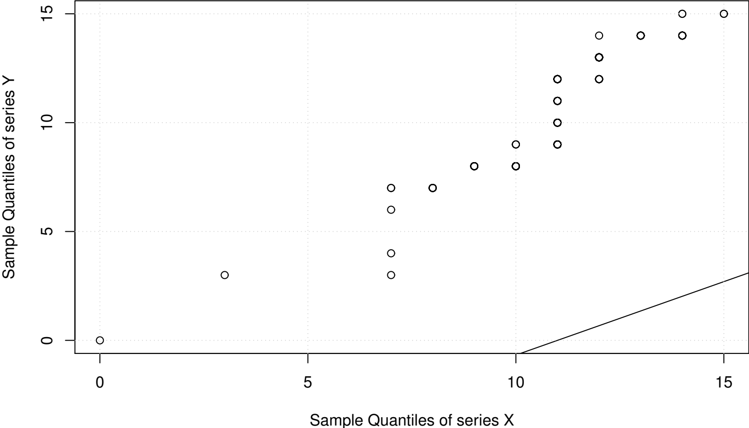
Q-Q Plot (series X vs Y)
