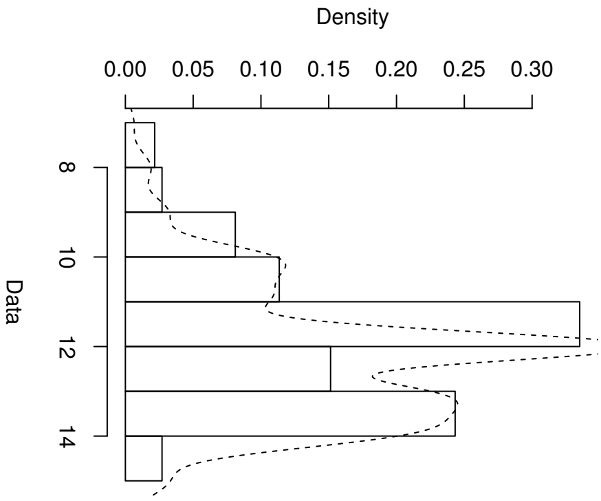
Empirical density
