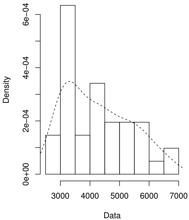
Empirical density
