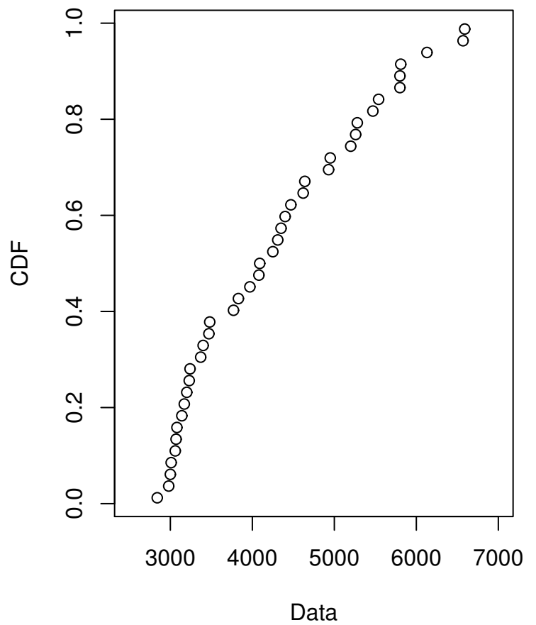
Cumulative distribution
