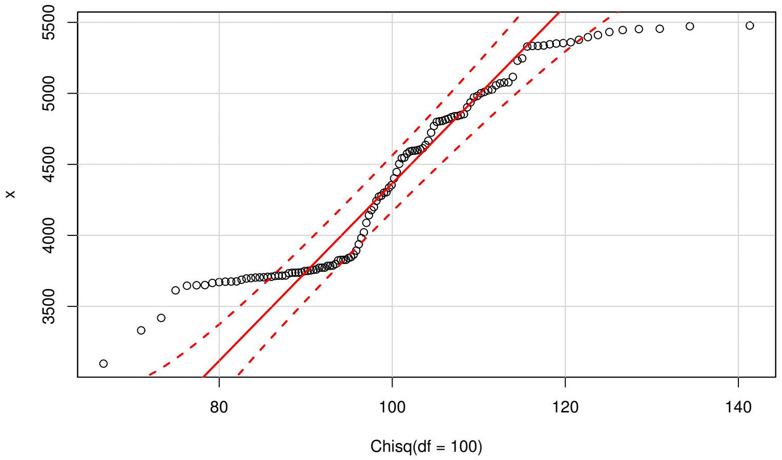
QQ plot (Chi-squared 1 param.)
