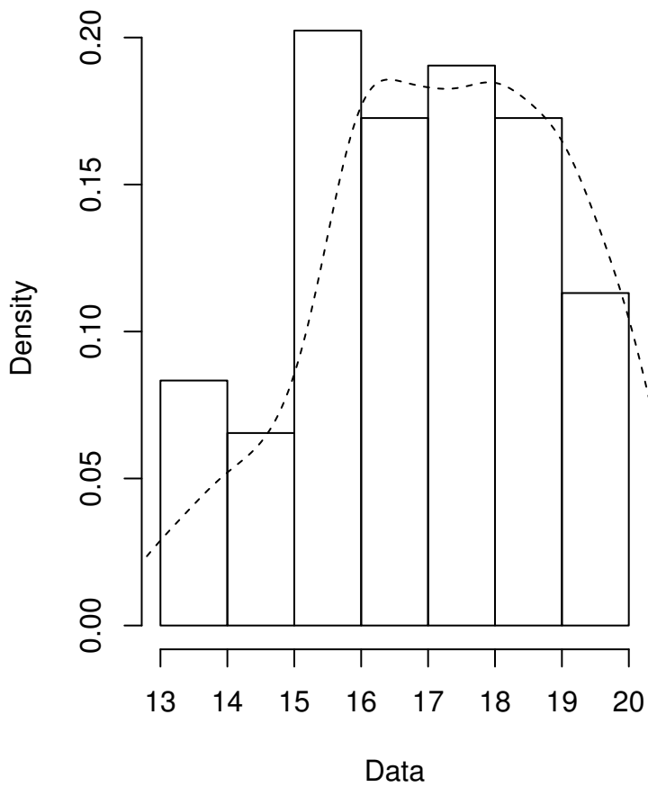
Empirical density
