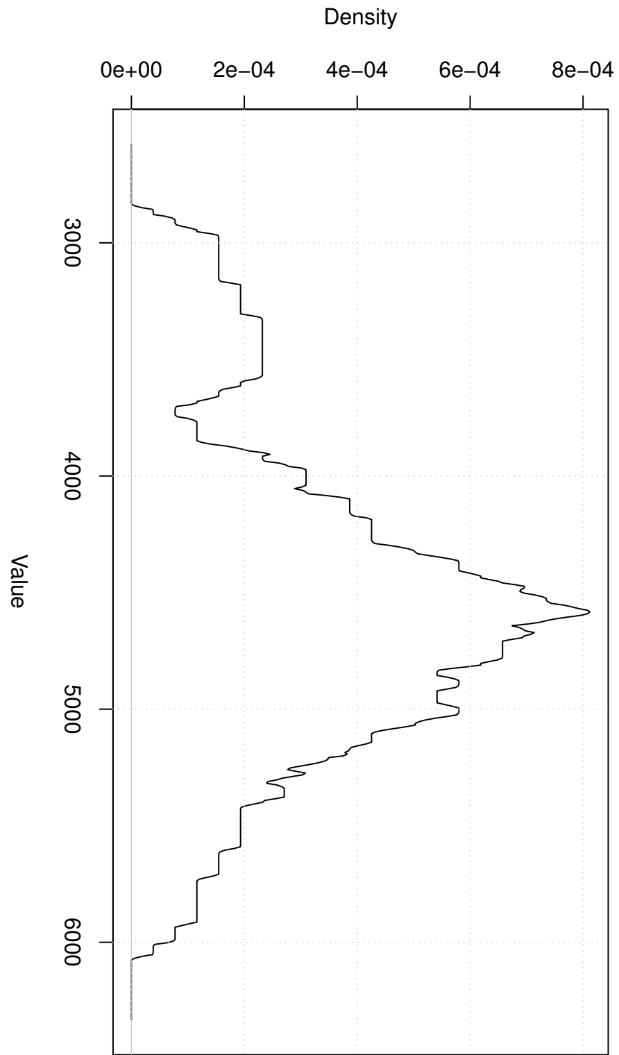
Rectangular Kernel
