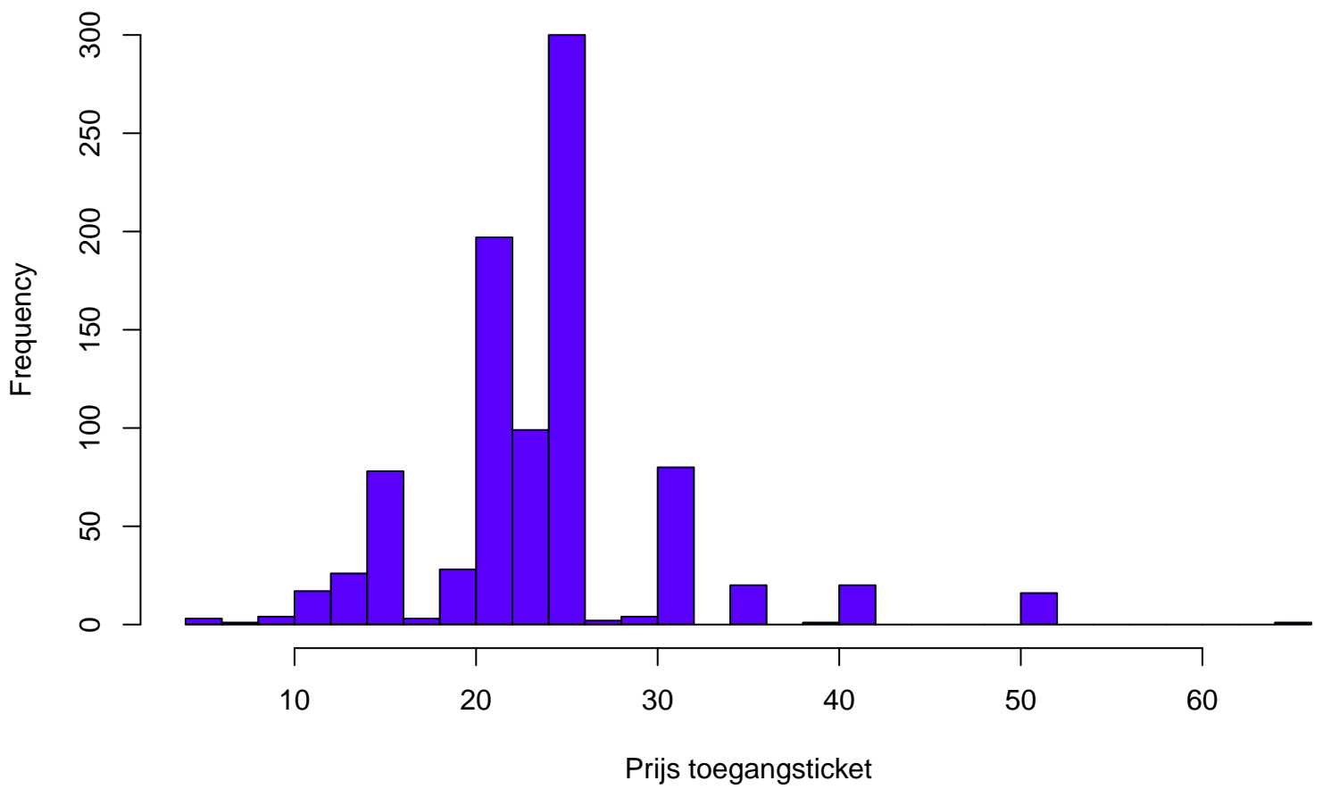
Histogram
