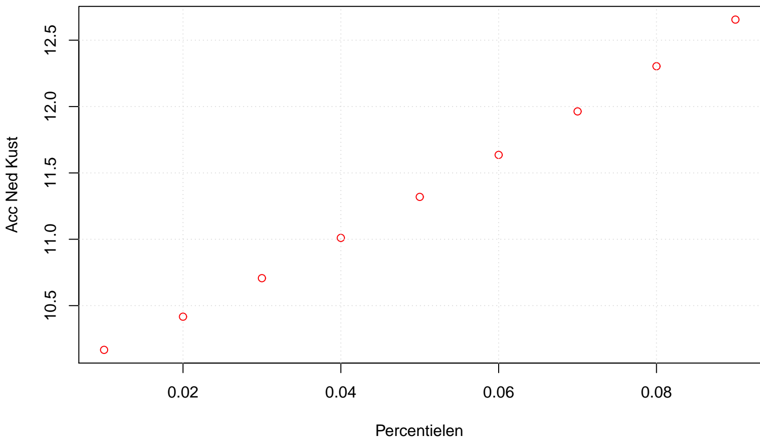
Harrell-Davis Quantiles Acc Ned Kust
