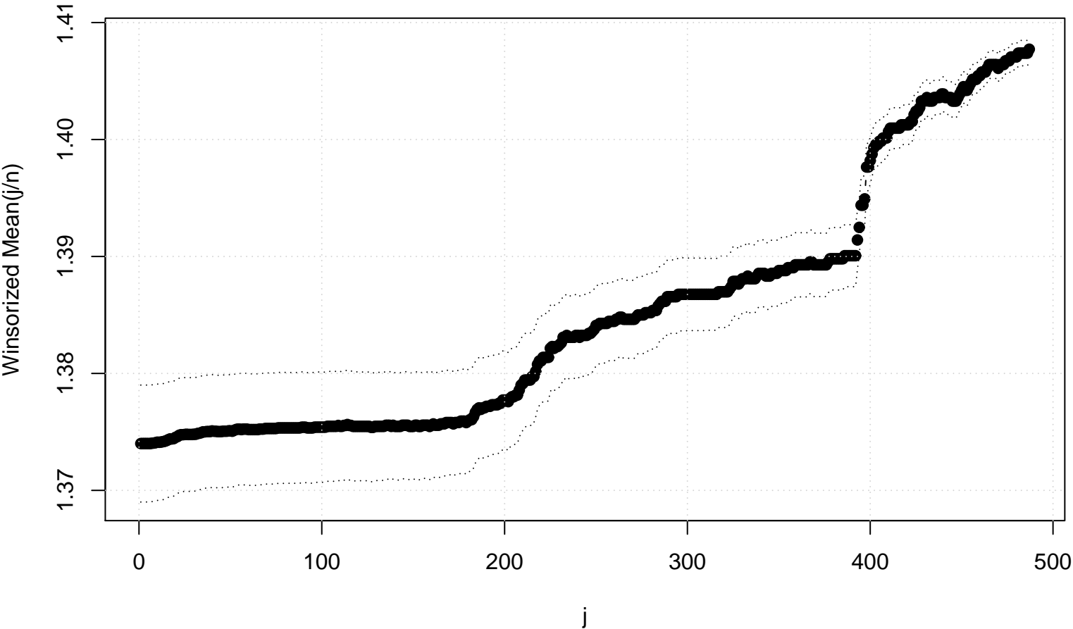
Robustness of Central Tendency
