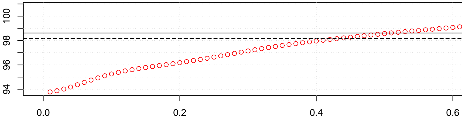
Harrell-Davis Quantiles
