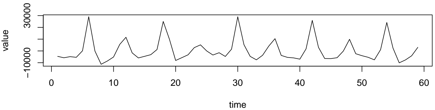
Working Time Series (lambda=1, d=1, D=0)
