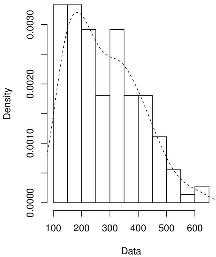
Empirical density
