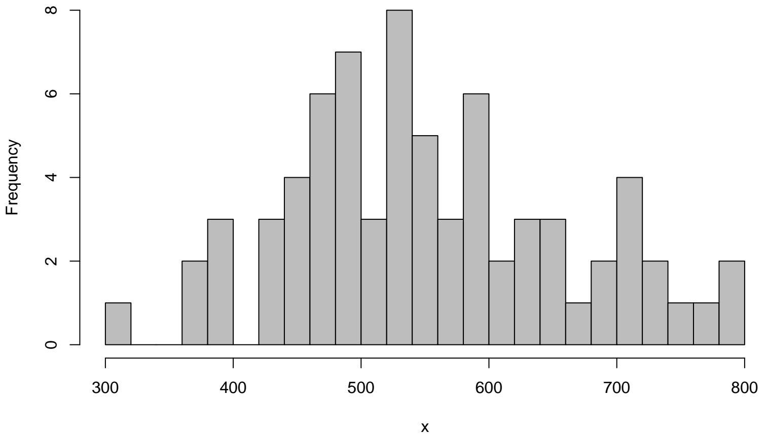
Histogram Faillissements 2010–2015
