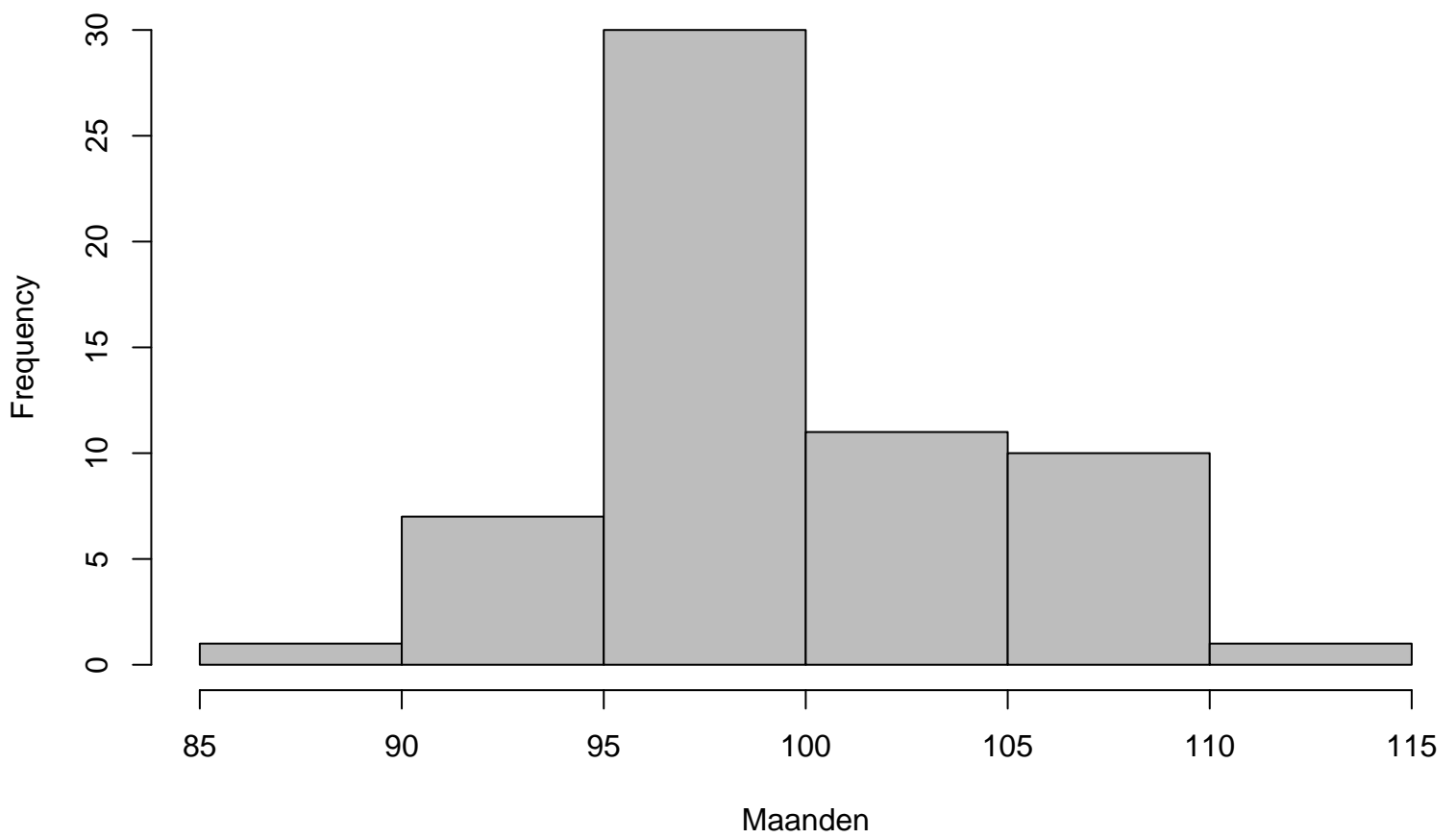
Histogram CPI
