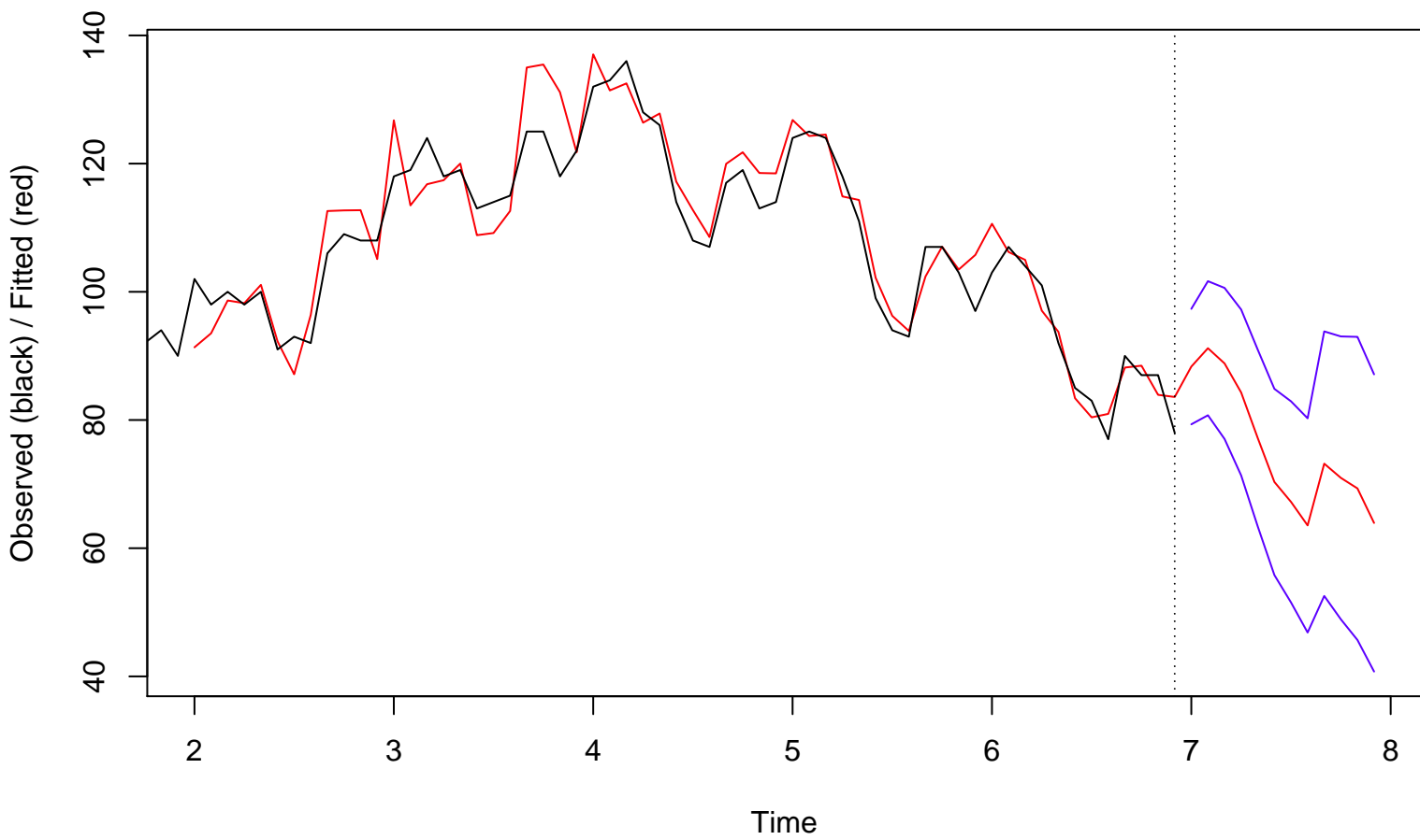
Extrapolation Fit of Exponential Smoothing
