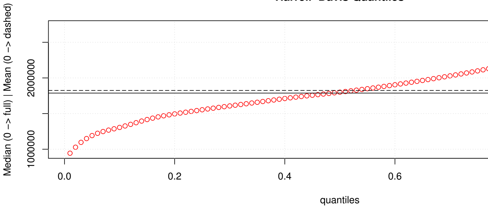
Harrell-Davis Quantiles
