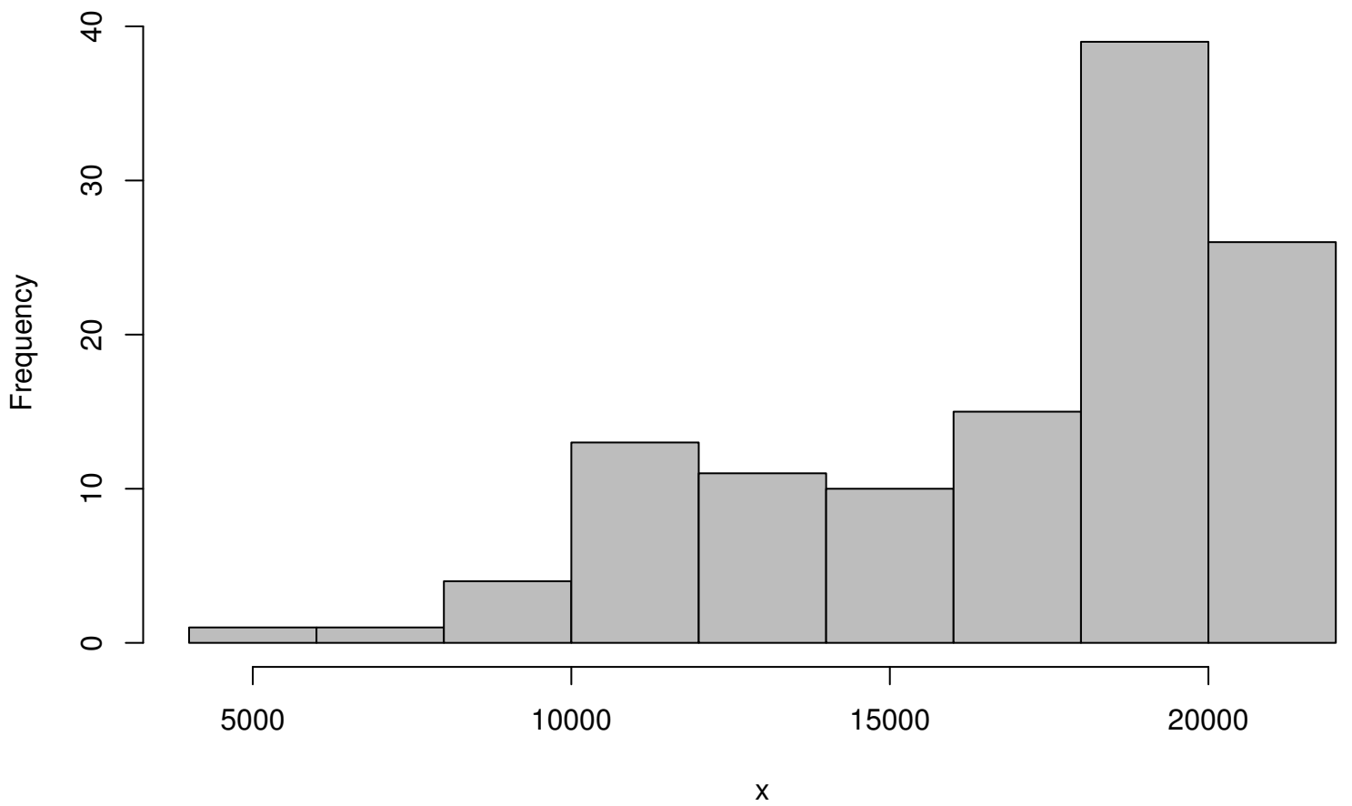
Histogram
