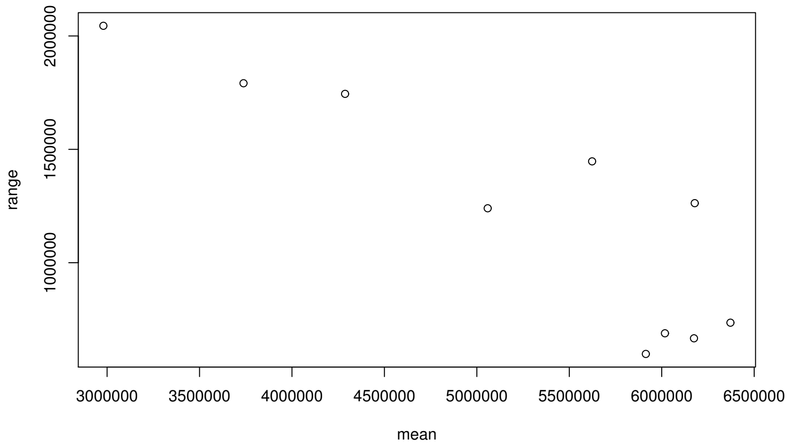
Range–Mean Plot
