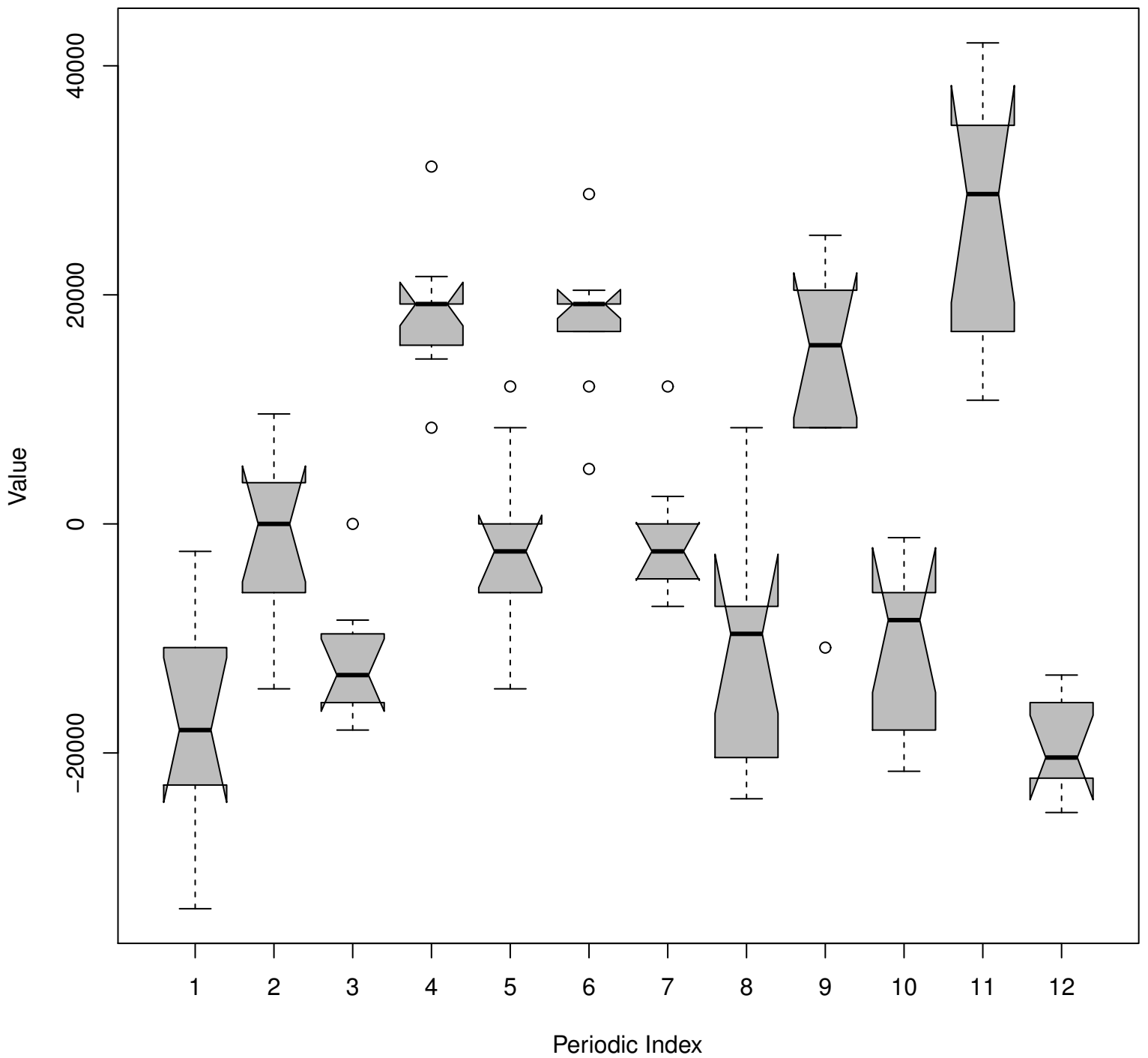
Notched Box Plots – Differenced Periodic Subseries
