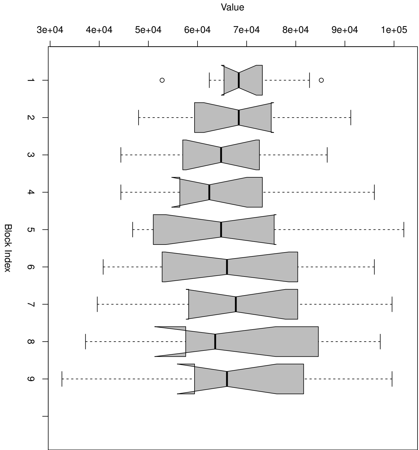
Notched Box Plots – Sequential Blocks
