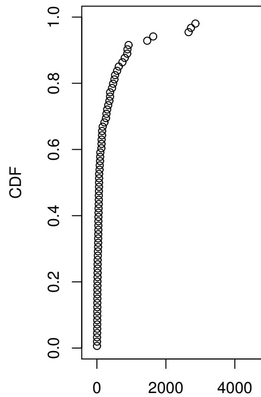
Cumulative
