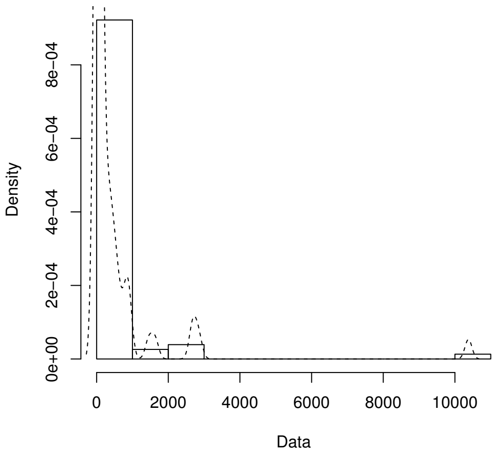
Empirical density
