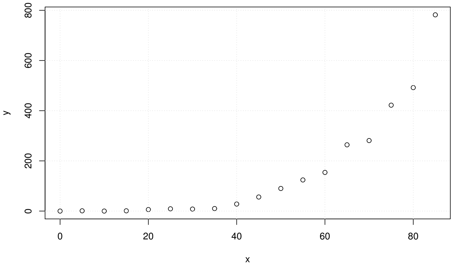
Scatterplot
