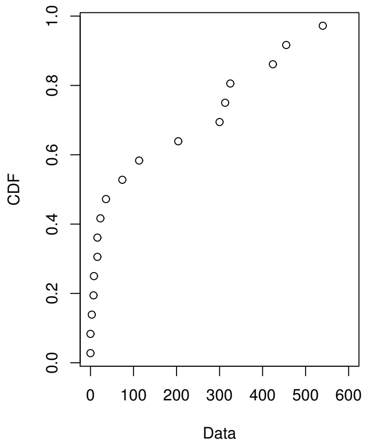
Cumulative distribution
